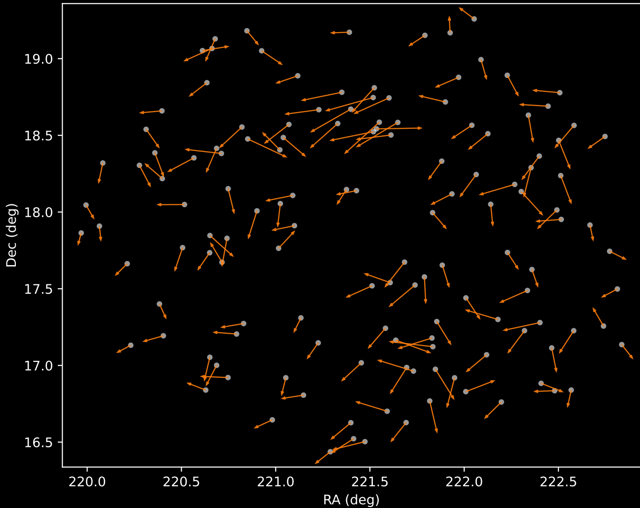
APOGEE DR17 Cluster 2 Proper Motion Vectors (n=136)
