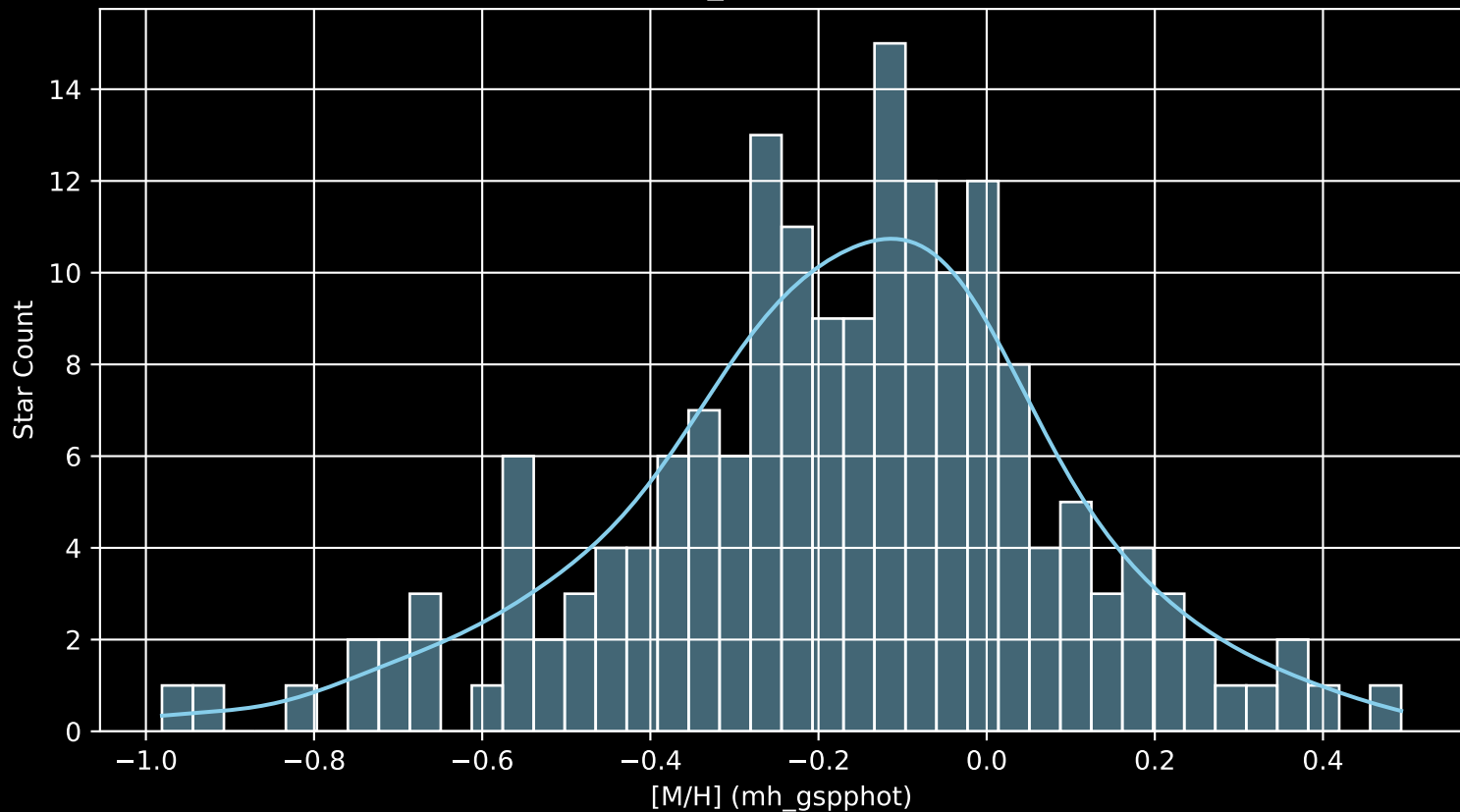
APOGEE DR17 Field: [204+24_MGA [M/H] (mh_gspphot) (n= 175)
