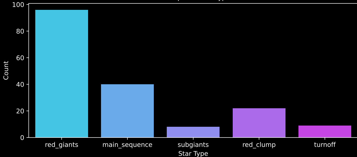
APOGEE DR17 Field: [204+24_MGA] Count plot of Star Type
