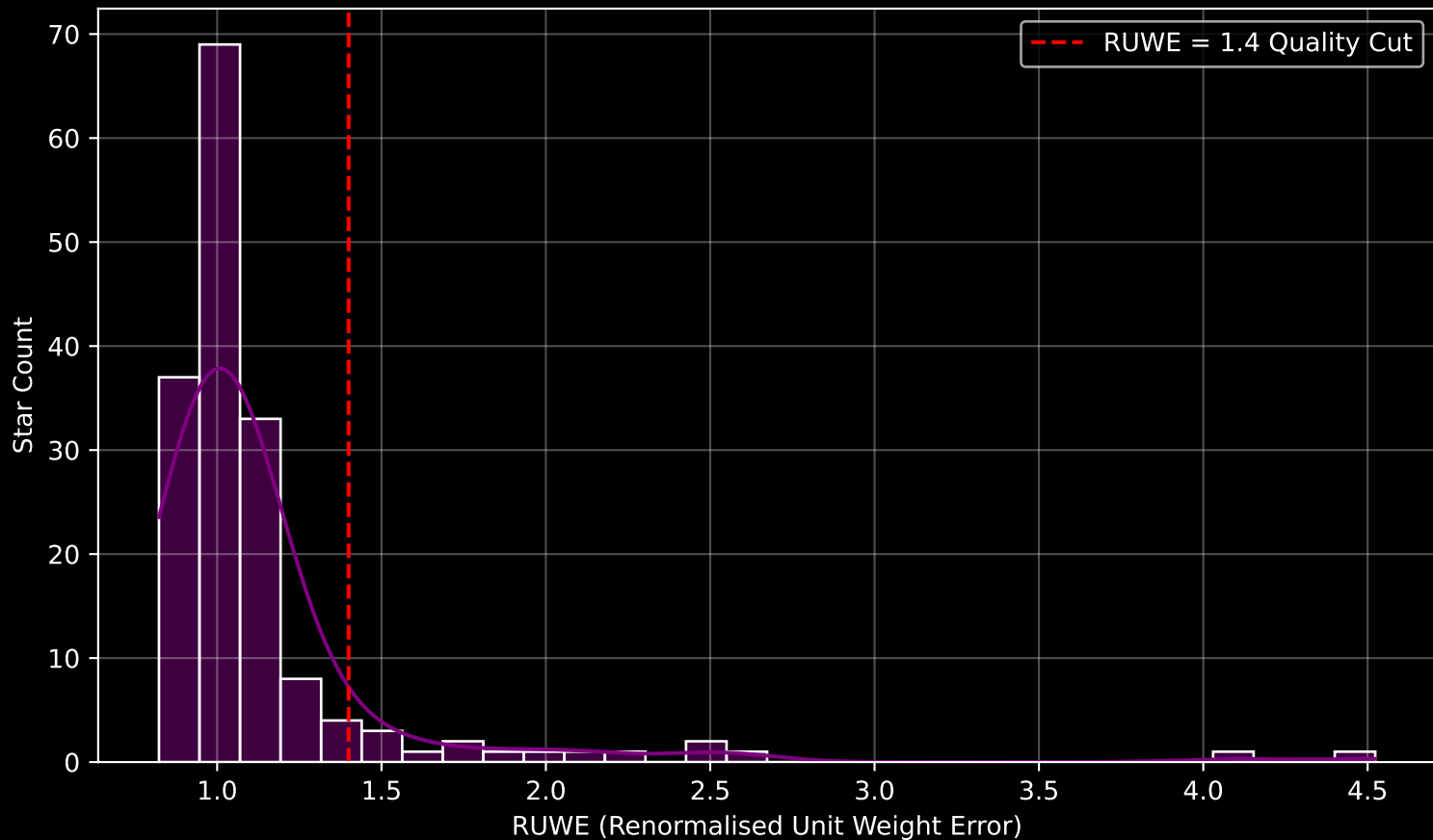
GAPOGEE DR17 Field [204+24_MGA] RUWE Distribution (n= 166)
