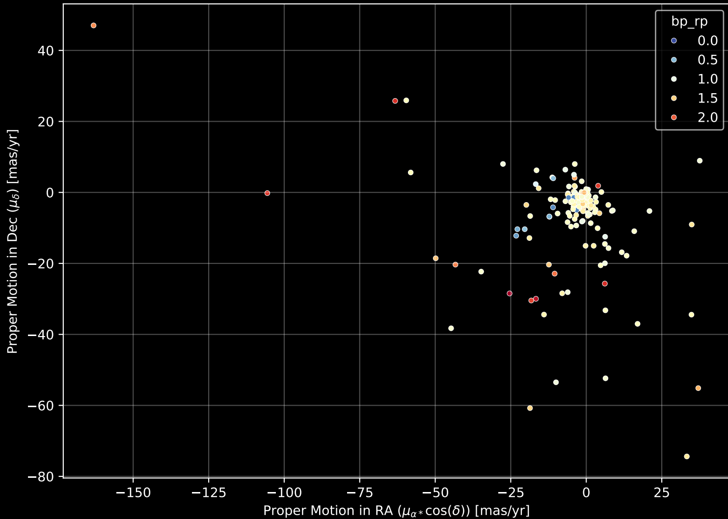
APOGEE DR17 Field: [204+24_MGA] Proper Motion Diagram (n= 175)
