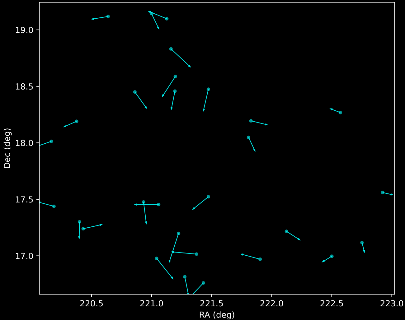
APOGEE DR17 Noise Stream Proper Motion Vectors (n=29)
