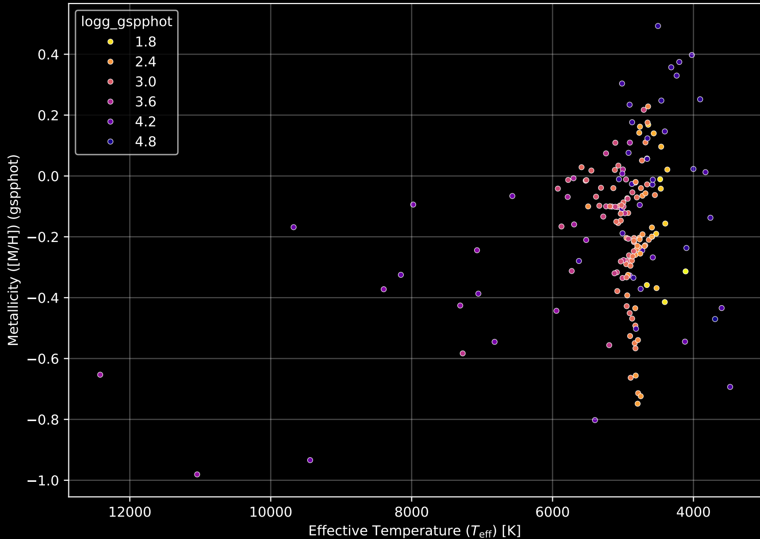
APOGEE DR17 Field: [204+24_MGA] Stellar Population Parameters (n= 175)
