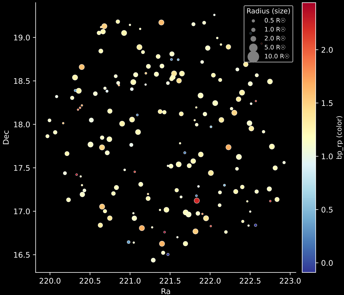
APOGEE DR17 Field: [204+24_MGA] Stars: 175
