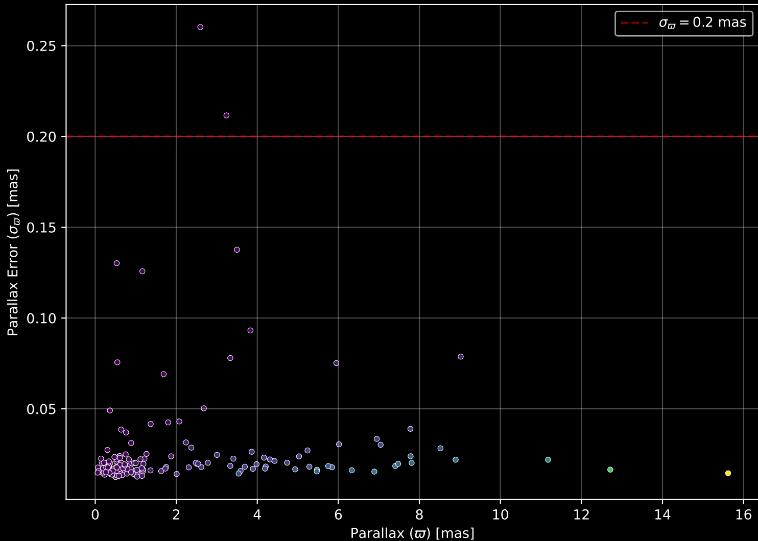
APOGEE DR17 Field: [204+24_MGA] Parallax Quality (n= 175)
